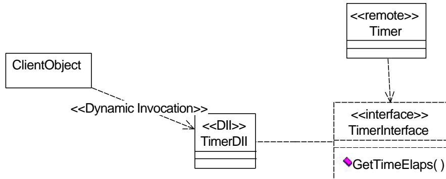
Figure 5. CORBA Version of Example
